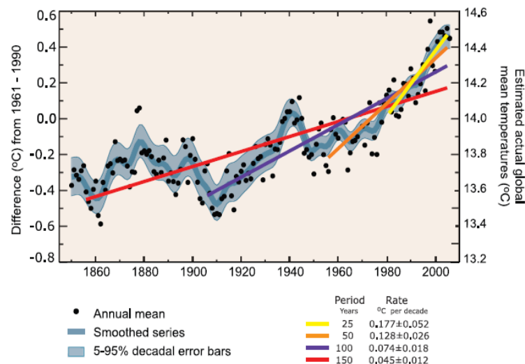
Figure TS.6. (Top) Patterns of linear global temperature trends over the period 1879 to 2005 estimated at the surface (left), and for the troposphere from satellite records (right). Grey indicates areas with incomplete data. (Bottom) Annual global mean temperatures (black dots) with linear fits to the data. The left hand axis shows temperature anomalies relative to the 1961 to 1990 average and the right hand axis shows estimated actual temperatures, both in °C. Linear trends are shown for the last 25 (yellow), 50 (orange), 100 (magenta) and 150 years (red). The smooth blue curve shows decadal variations (see Appendix 3.A), with the decadal 90% error range shown as a pale blue band about that line. The total temperature increase from the period 1850 to 1899 to the period 2001 to 2005 is 0.76^{\circ}\text{C} \pm 0.19^{\circ}\text{C} . [FAQ 3.1, Figure 1.]
